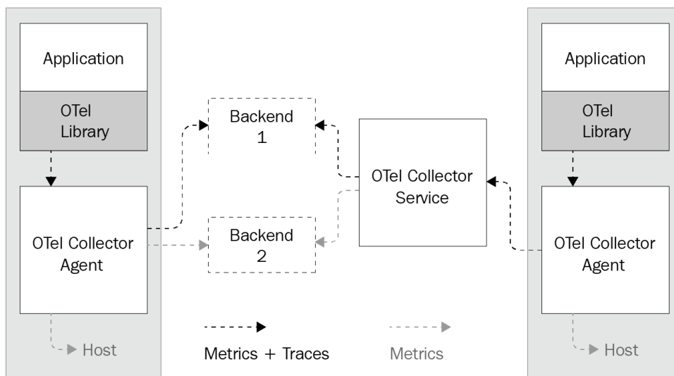
Figure 9.1 – OpenTelemetry reference architecture
