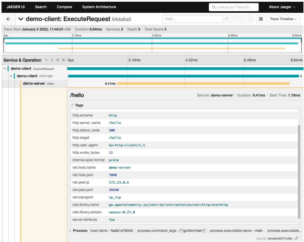
Figure 9.3 – The Jaeger client/server-distributed trace
