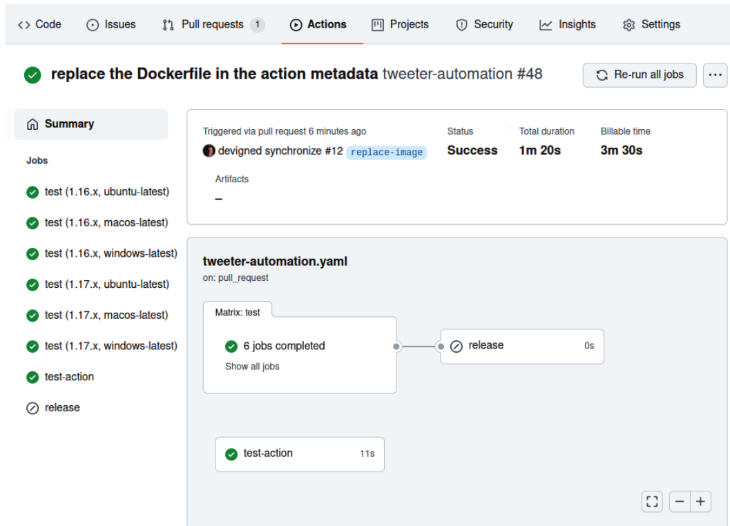
Figure 10.12 – The workflow view showing the speed increase of the test-action job
