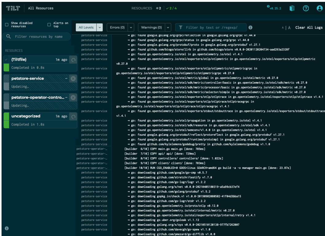
Figure 14.2 – Tilt's All Resources web view
