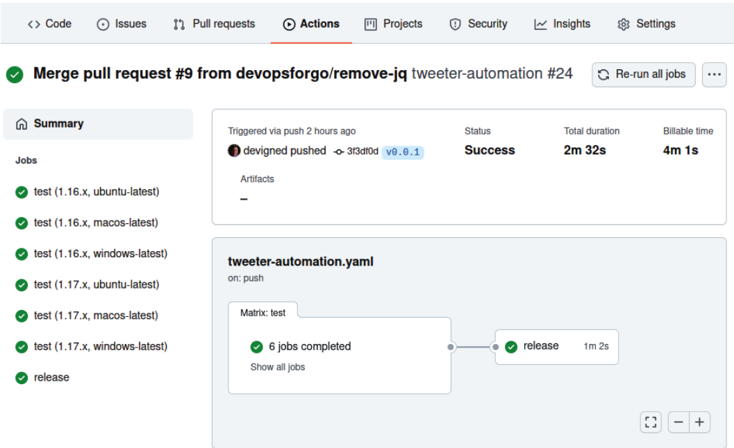
Figure 10.5 – The workflow job view showing dependent test and release jobs
