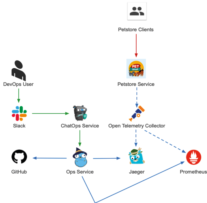
Figure 11.1 – ChatOps and Petstore architecture
