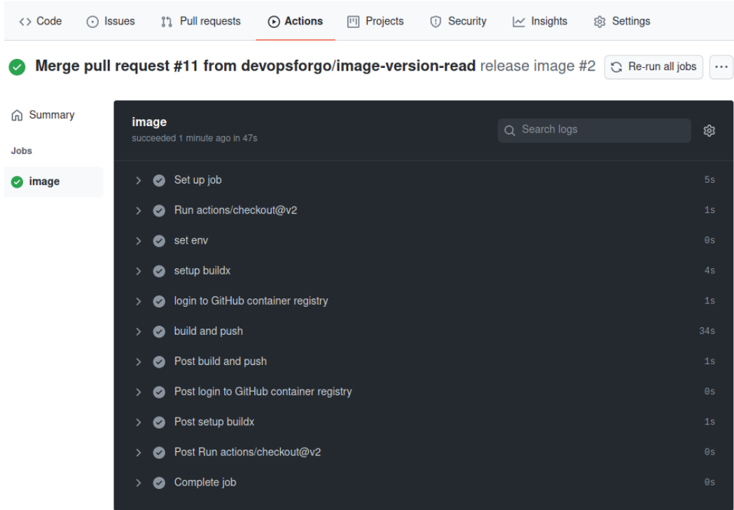
Figure 10.11 – The image release job output
