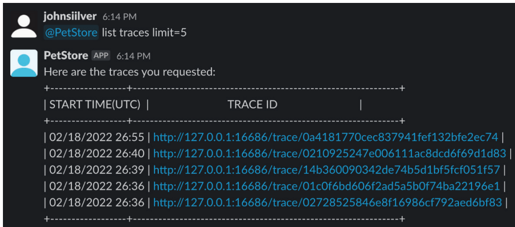
Figure 11.13 – Output from a command to list the last five traces
