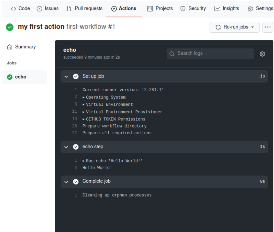
Figure 10.3 – The echo job output view
