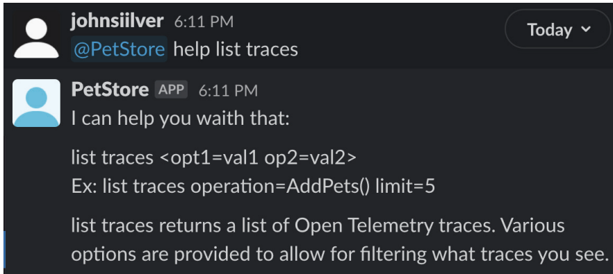
Figure 11.12 – Help output for the list traces command
