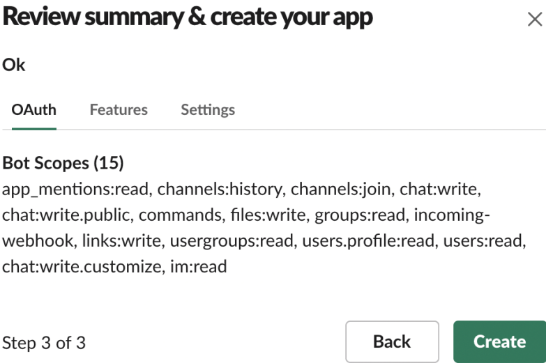
Figure 11.6 – Bot creation summary
