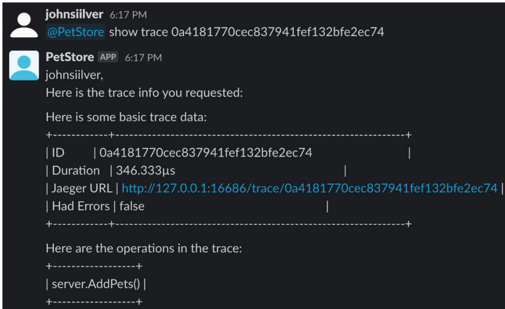
Figure 11.14 – Output showing a specific trace's data
