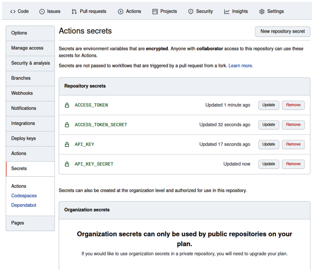
Figure 10.13 – Repository secrets
