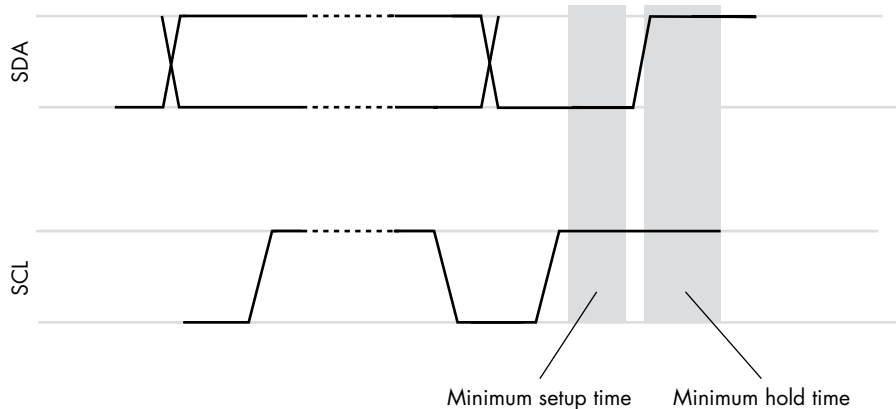
Figure 2-4: I 2 C stop condition ( S_P )
