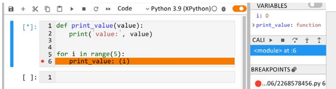
Figure 11.3: Debugging using Jupyter
