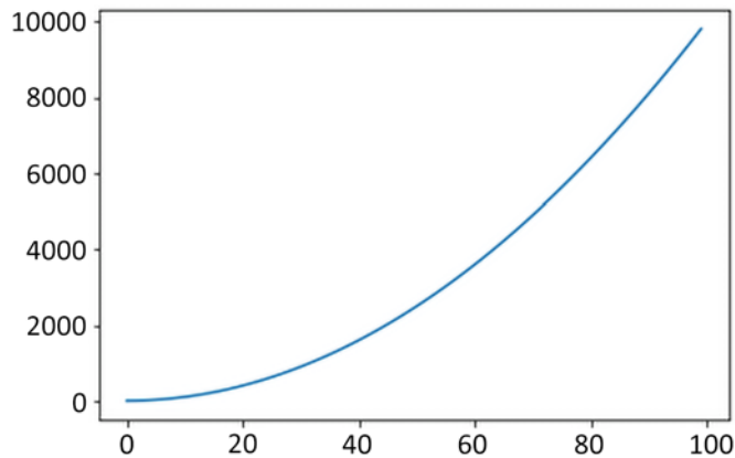
Figure 15.1: Matplotlib plot
