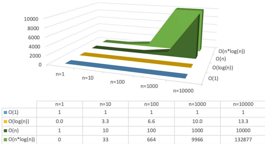
Figure 4.1: Time complexity of slow-growing functions with n=1 to n=10,000
