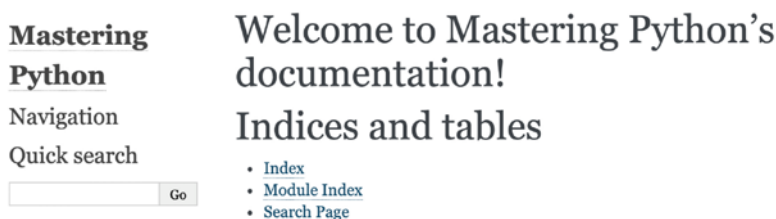
Figure 9.19: Viewing index.html
