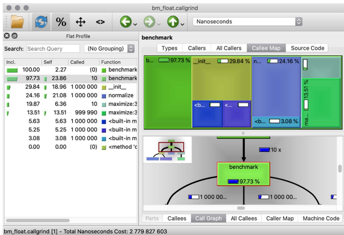
Figure 12.1: QCacheGrind
